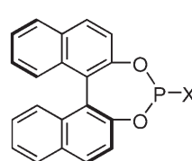
1a X = OR 1b X = alkyl or aryl 1c X = NR 2 , MonoPhos
