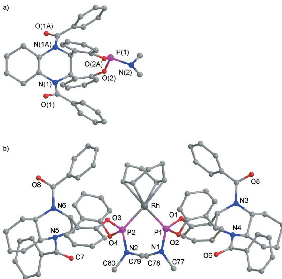
Figure 1. Crystal structure of 4b (top) and [\text{Rh}\{\mathbf{4b}\}_2(\text{cod})]^+ \text{BF}_4^- (bottom). The \text{BF}_4^- anion and all hydrogen atoms have been omitted for clarity. Selected interatomic distances [Å], angles, and torsion angles [°] in ligand 4b : P(1)–N(2) 1.711(4), P(1)–O(2) 1.456(3), P(1)–O(2 A) 1.492(3); and [\text{Rh}\{\mathbf{4b}\}_2(\text{cod})]^+ \text{BF}_4^- : Rh–P(1) 2.296(3), Rh–P(2) 2.302(3), P(1)–N(1) 1.647(13), P(2)–N(2) 1.625(14); P(1)–O(1) 1.624(9), P(1)–O(2) 1.640(10), P(2)–O(3) 1.622(10), P(2)–O(4) 1.651(10); P(1)–Rh–P(2) 95.96(11), P(1)–Rh–P(2)–N(2) 27.1(6), P(2)–Rh–P(1)–N(1) 29.6(6).
