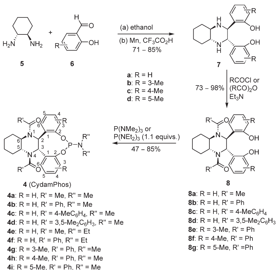
Scheme 1. Synthesis of monodentate ligands 4a–i .
